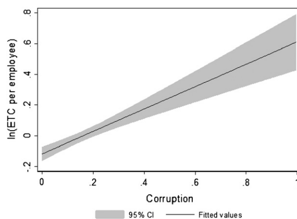
Fig. 3. The relationship between corruption and ETC.
